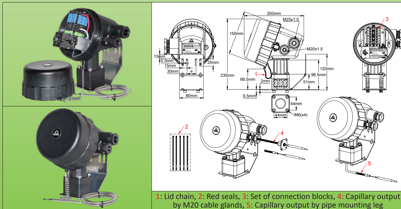
1: Lid chain, 2: Red seals, 3: Set of connection blocks, 4: Capillary output by M20 cable glands, 5: Capillary output by pipe mounting leg
