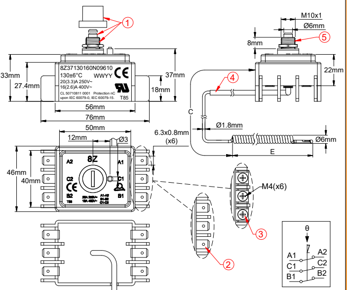
Mounting by M10×1 front bushing or mounting brackets, horizontal terminals, type 8Z31 and 8Z37
